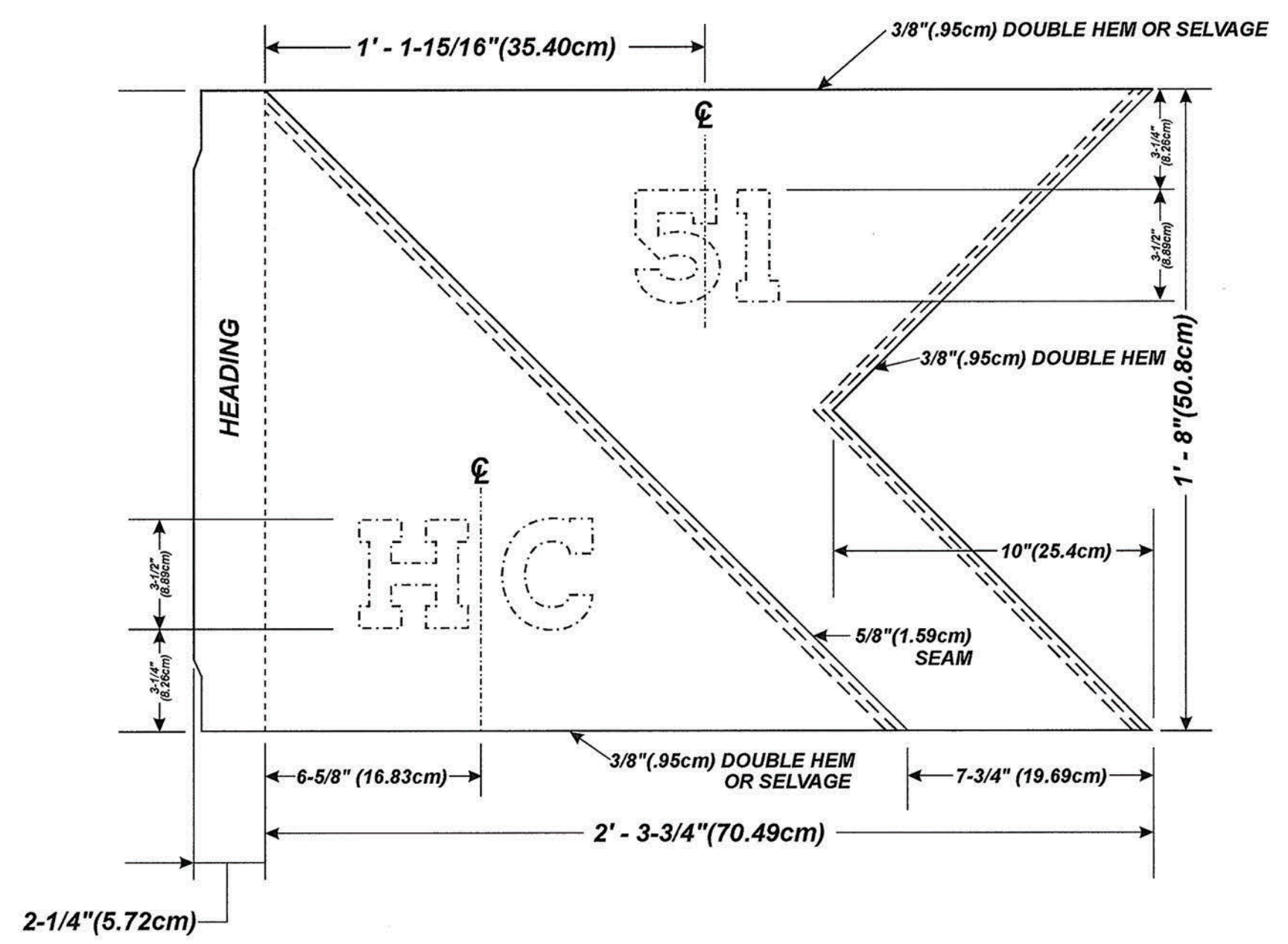
GUIDON, HEADQUARTERS COMPANY/DETACHMENT SCALE: 3" = 1' - 0"
