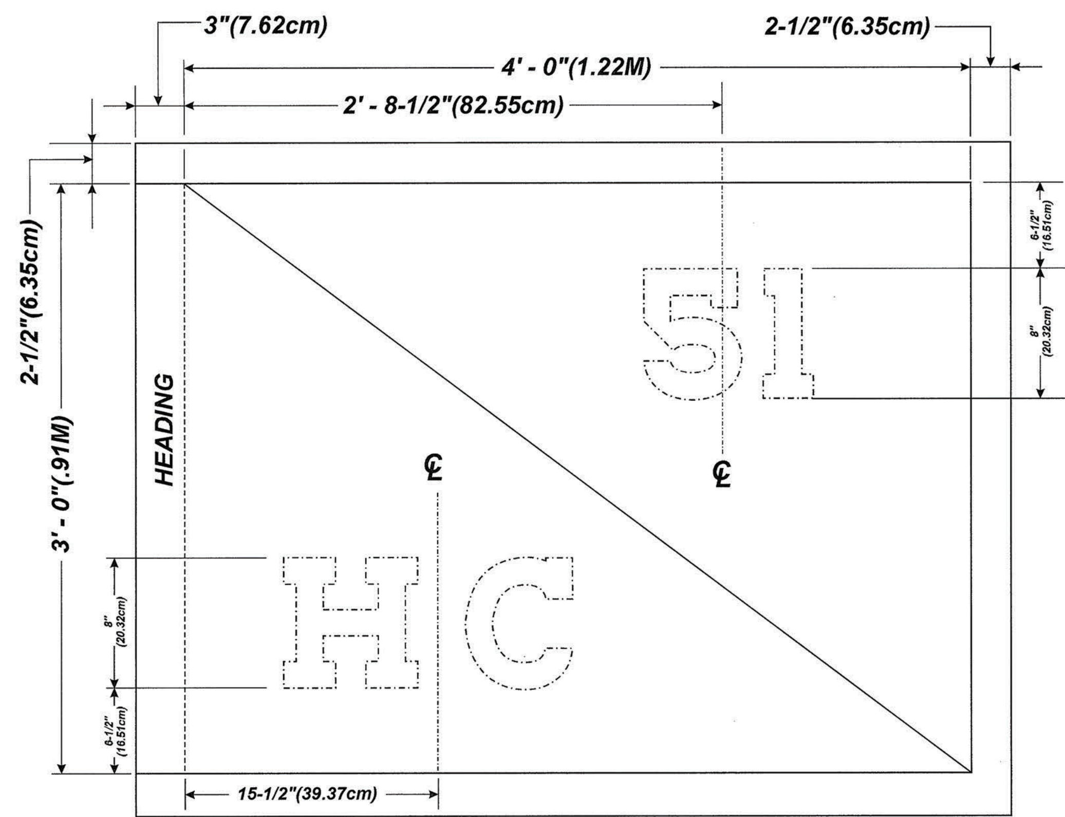
DISTINGUISHING FLAG, HEADQUARTERS SCALE: 2" = 1' - 0"
